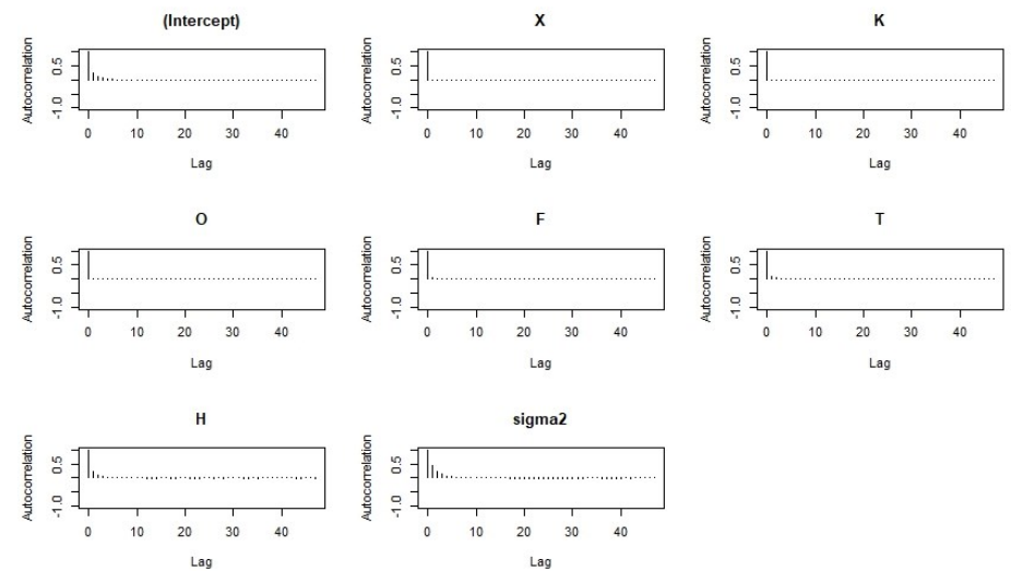
Figure 4: Autocorrelation plots
